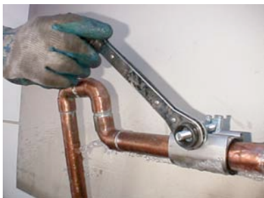
Tighten bolt
