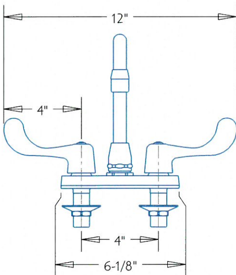
WRISTBLADE HANDLES
